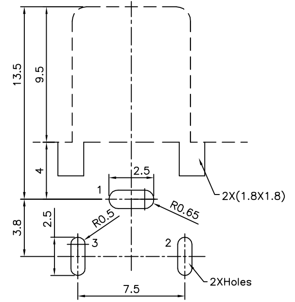
Recommended P.C.B. Layout(Printed-Side View) Thickness=1.6mm(PCB Board Tolerance±0.1)
