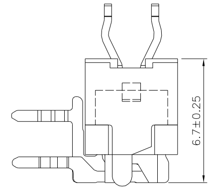
Mating Height Draw.
