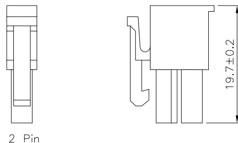
2 Pin
