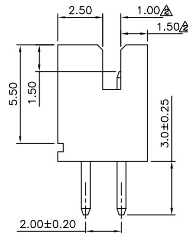
△04 Pin Configuration
