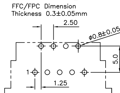
Recommended P.C.B. Layout Component Side
