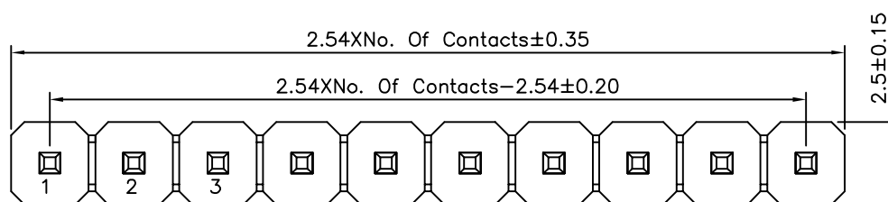
Recommended P.C.B. Layout(Top View) (PCB Board Tolerance±0.05)
