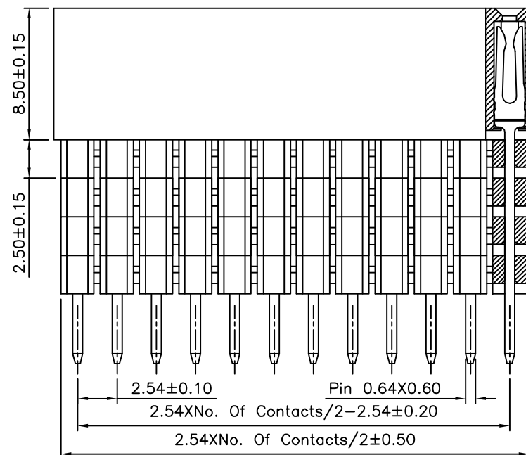
Section K-K
