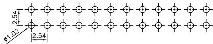
Recommended P.C.B. Layout (Top Side) (PCB Board Tolerance \pm 0.05 )
