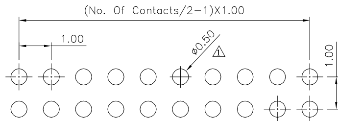
3 Recommended P.C.B. Layout
