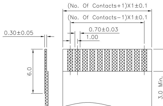
Applicable FPC/FFC Thickness:0.25~0.35mm
