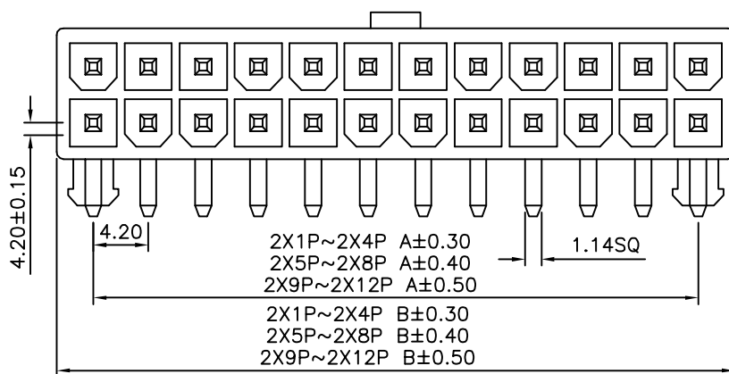
2X3Pin~2X12Pin
