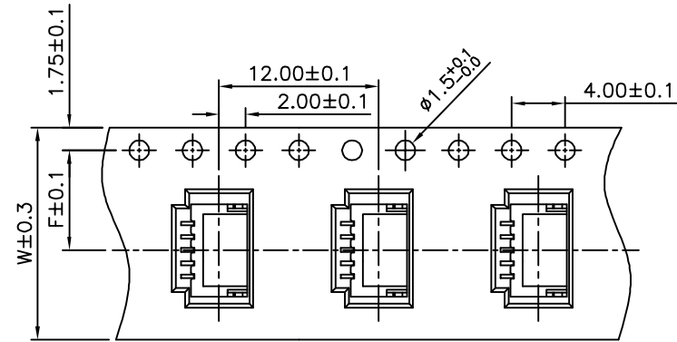
2~13 Contacts
