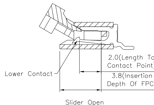
Applicable FPC/FFC Thickness 0.25~0.35mm
