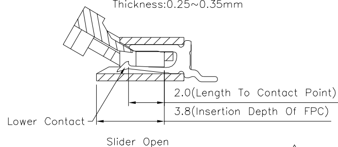
Applicable FPC/FFC Thickness:0.25~0.35mm
