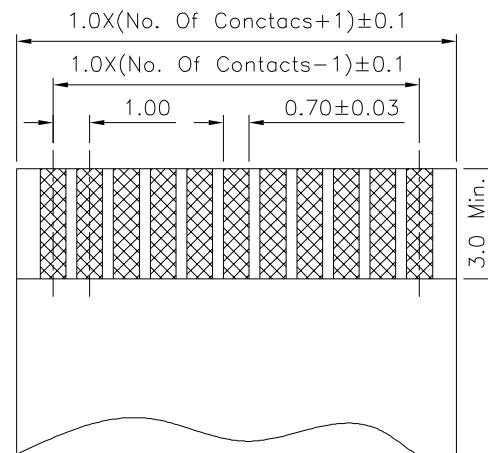
Applicable FPC/FFC Thickness:0.25~0.35mm
