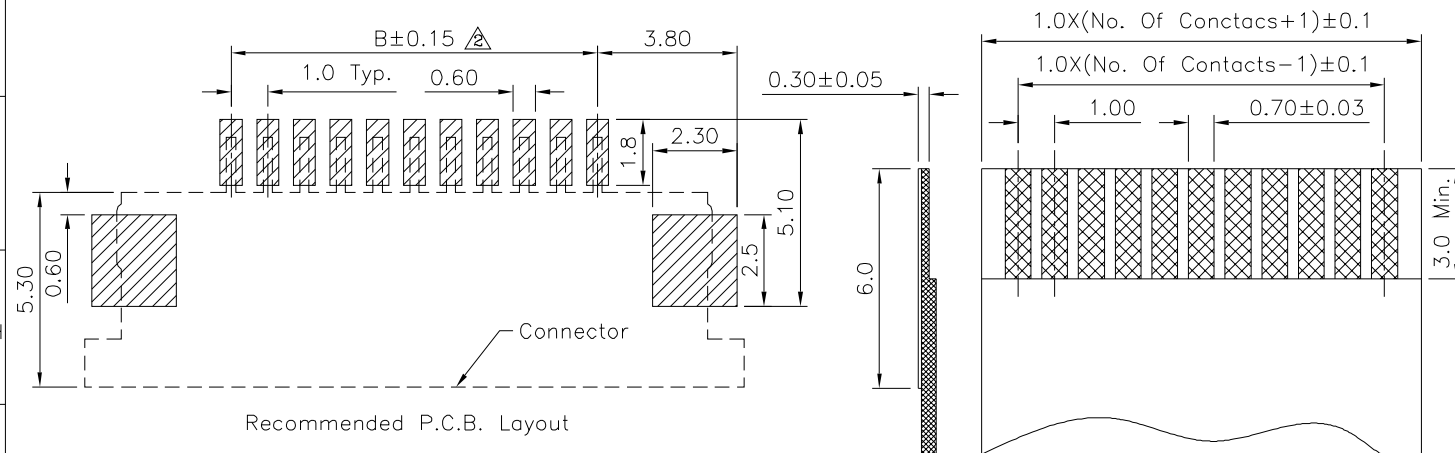
Applicable FPC/FFC Thickness:0.25~0.35mm
