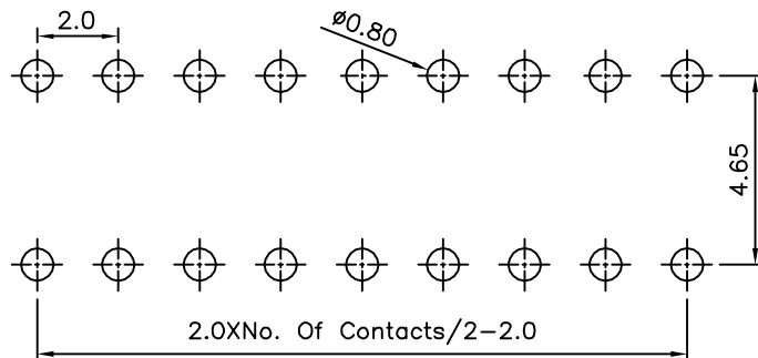
Recommended P.C.B. Layout(Top View) (PCB Board Tolerance \pm 0.05 )
