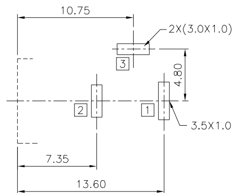
Recommended P.C.B. Layout(Bottom View) (PCB Board Tolerance±0.05)
