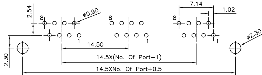
△ PC Board Layout Ref.
