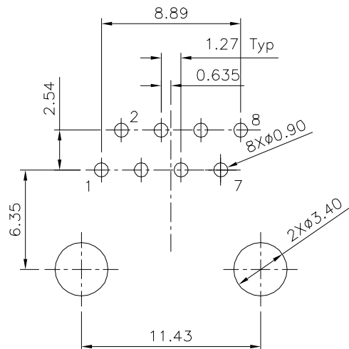
△ Recommended P.C.B. Layout(Top View) (PCB Board Thickness:1.6mm)Tolerance±0.05
