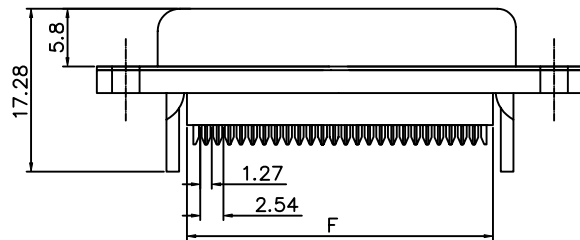
With Insulator Support
