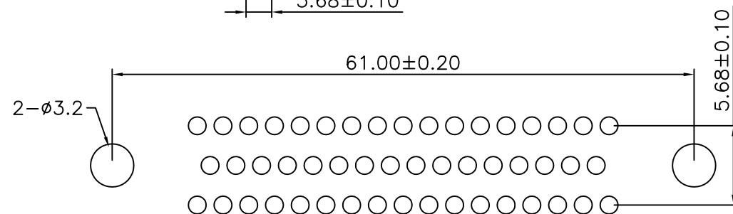
PCB Layout
