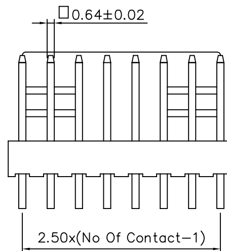
(6 Through 20 Circuits)
