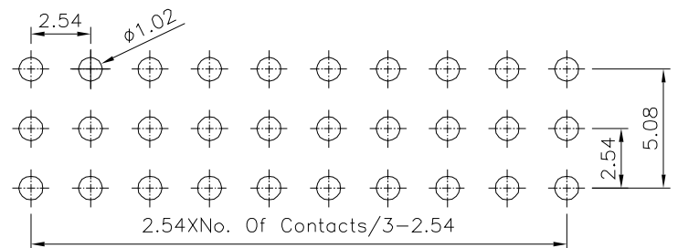
Recommended P.C.B. Layout(Top View) (PCB Board Tolerance±0.05)
