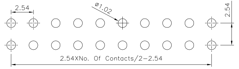
Recommended P.C.B. Layout(Top View) (PCB Board Tolerance±0.05)
