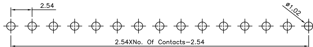
Recommended P.C.B. Layout(Top View) (PCB Board Tolerance±0.05)
