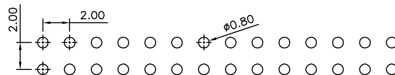
Recommended P.C.B Layout(Top Side) (PCB Board Tolerance±0.05)
