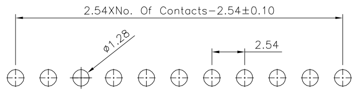
Recommended P.C.B. Layout Tolerance ±0.05
