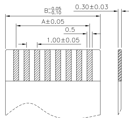
Accommodated FFC/FPC
